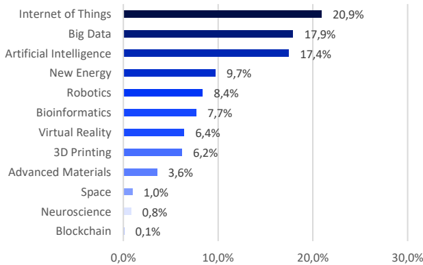
Singularity Sectors
